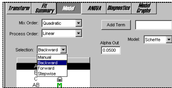
Modified Mix Order (Quadratic) and Selection Criteria (Backward)
