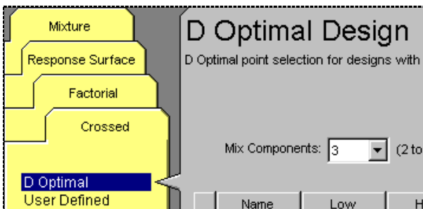
D Optimal Design Option for Crossed Design
