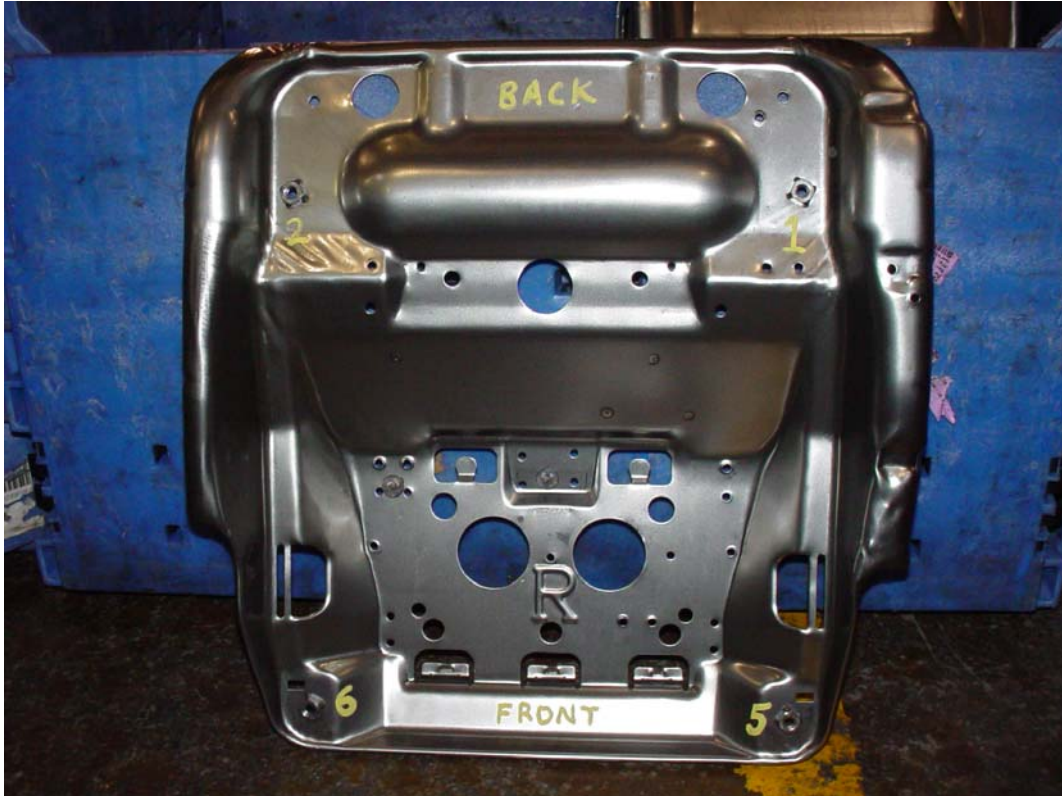
Figure 1: Seat pan with four weld joints marked with yellow numbers.
