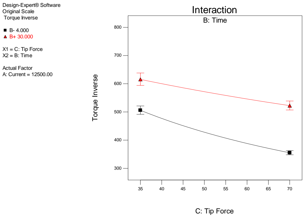
Figure 3: Interaction between time and tip force
